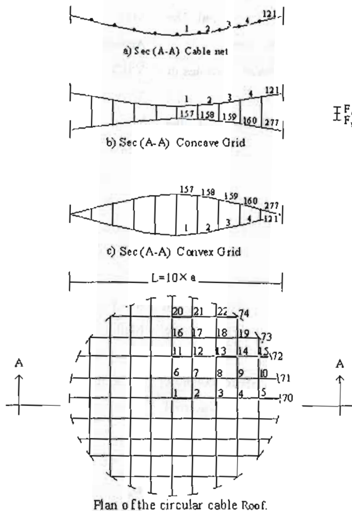
Fig. (1): (10×10) Circular cable roof.
