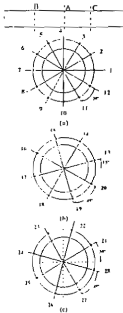
Fig. (5) Distribution of the thermocouples probes on the cylinder, (a) at the middle of the tube, (b) at the left end, and (c) at the right end.
