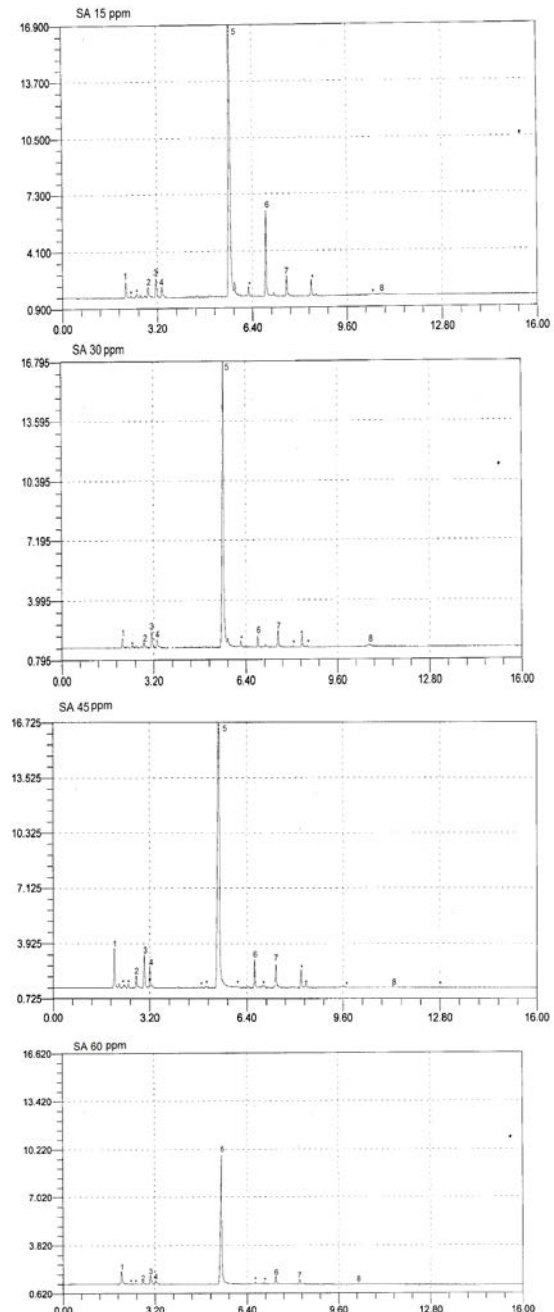
1= \alpha - pinene 2= Myrcene 3= B- pinene 4= \rho Cymene 5= Linalool 6= Borneol 7= Linalyl acetate 8= Geranyl acetate * = Unknown compounds
