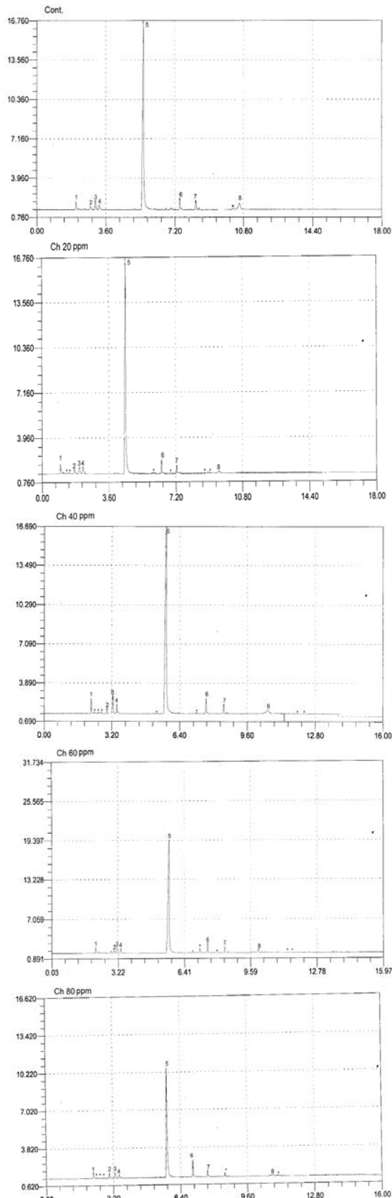
1= \alpha - pinene 2= Myrcene 3= B- pinene 4= \rho Cymene 5= Linalool 6= Borneol 7= Linalyl acetate 8= Geranyl acetate * = Unknown compounds
