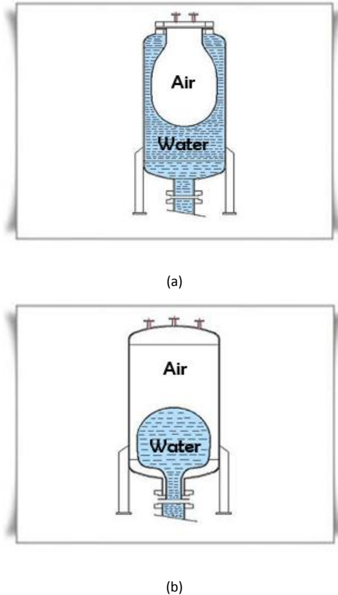
Fig.(3) :(a&b) Air vessels with bladders
