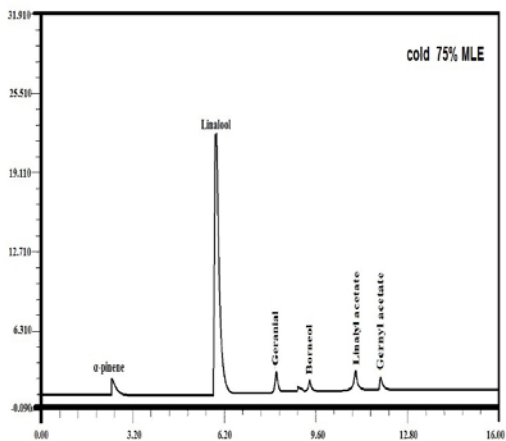
Figure 2. G.L.C chromatogram analysis of coriander oil constituents on the cold MLE extract 75% .
