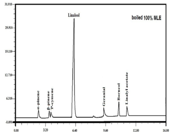
Figure 5. G.L.C. chromatogram analysis of coriander oil constituents on the boiled MLE extract 100% .
