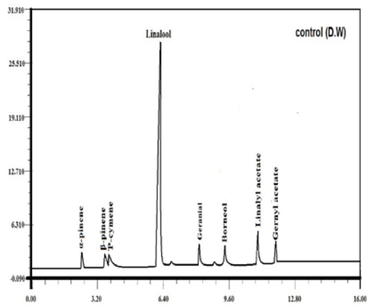
Figure 1. G.L.C. chromatogram analysis of coriander oil constituents (%) on the control (D.W).
