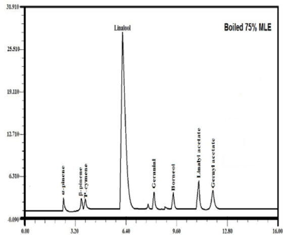
Figure 4. G.L.C chromatogram analysis of coriander oil constituents on the boiled MLE extract 75% .
