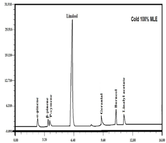
Figure 3. G. L.C. chromatogram analysis of coriander oil constituents on the cold MLE extract 100% .
