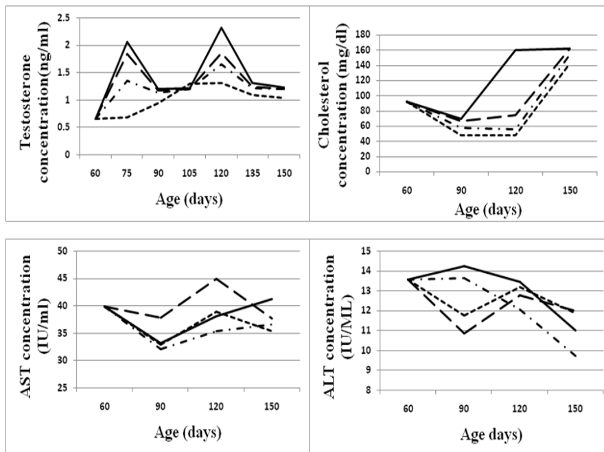
Figure 4: Plasma concentrations of testosterone and cholesterol, and activity of AST and ALT in blood plasma of male NZW rabbits orally administered with royal jelly or/ and bee honey and control rabbits.
