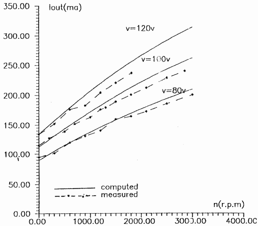
Fig.(7) The output current against prime-mover speed for different constant applied voltages
