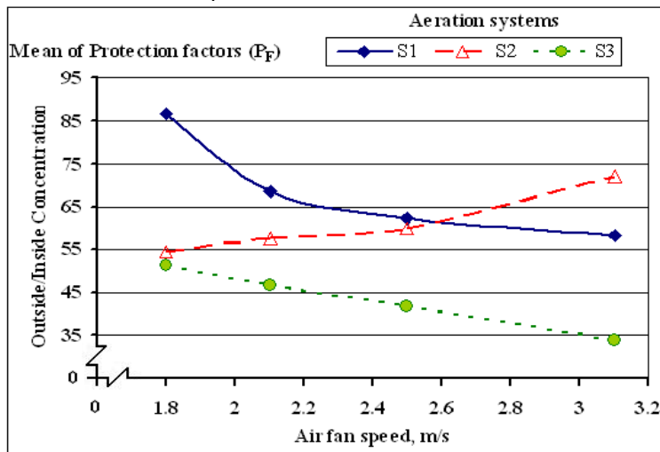
Fig. 15: Effect of Air fan speed on In - cab Protection factors of PM 2.5 at different aeration systems under study.
