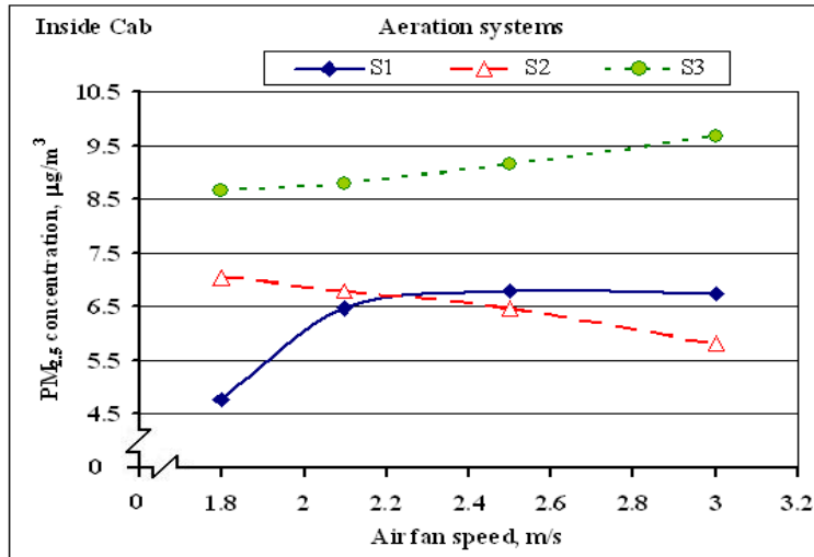
Fig. 14: Effect of Air fan speed on In - cab PM 2.5 concentration at different aeration systems under study.
