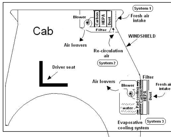
Fig. 1: Schematic diagram of a three systems of air flow through filters at the stationary cab.
