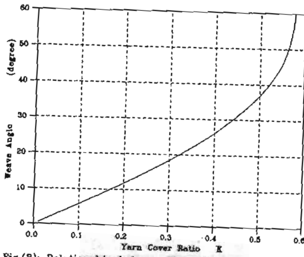
Fig.(3): Relationship between Yarn Cover Ratio and Weave Angle in Plain Square Fabric Woven from Flexible Yarns
