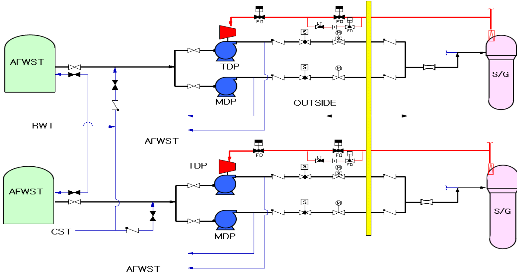
Figure4. Auxiliary feed water system (AFWS)
