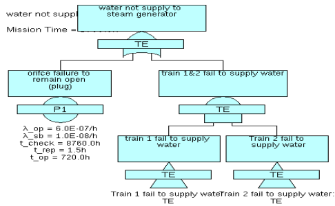
Figure 10. Fault tree construction.
