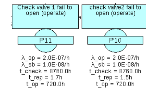
Figure17. Check valves failure.
