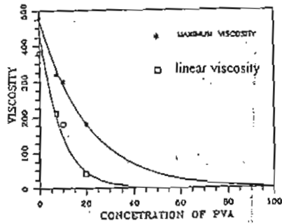
FIG ( 3 ) EFFECT OF ADDING PVA TO RICE STARCH ON VISCOSITY
