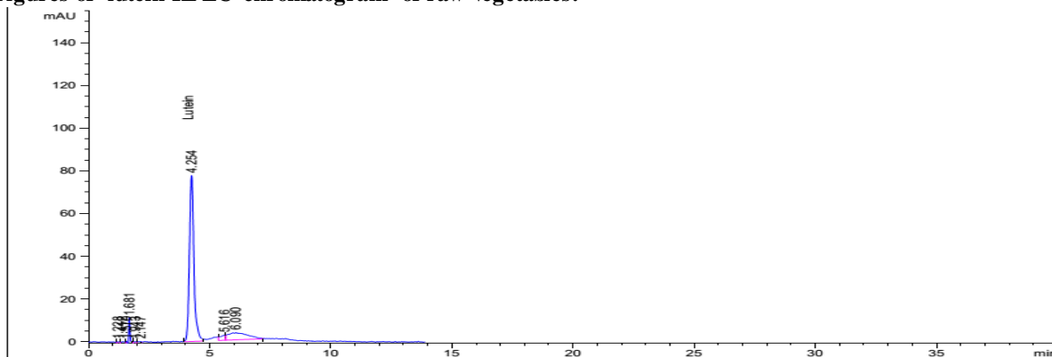
Fig. 1. HPLC chromatogram of standard lutein
