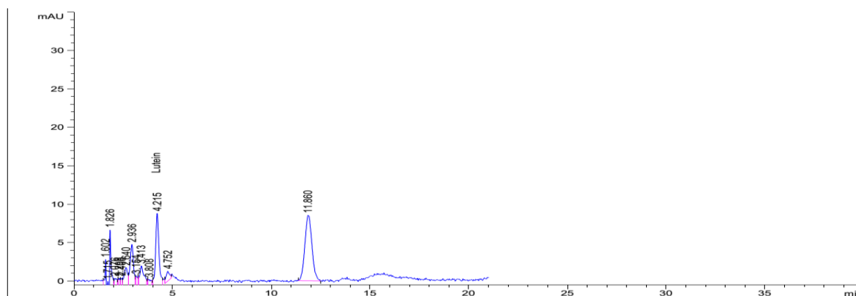
Fig. 4. HPLC chromatogram of lutein in parsley.
