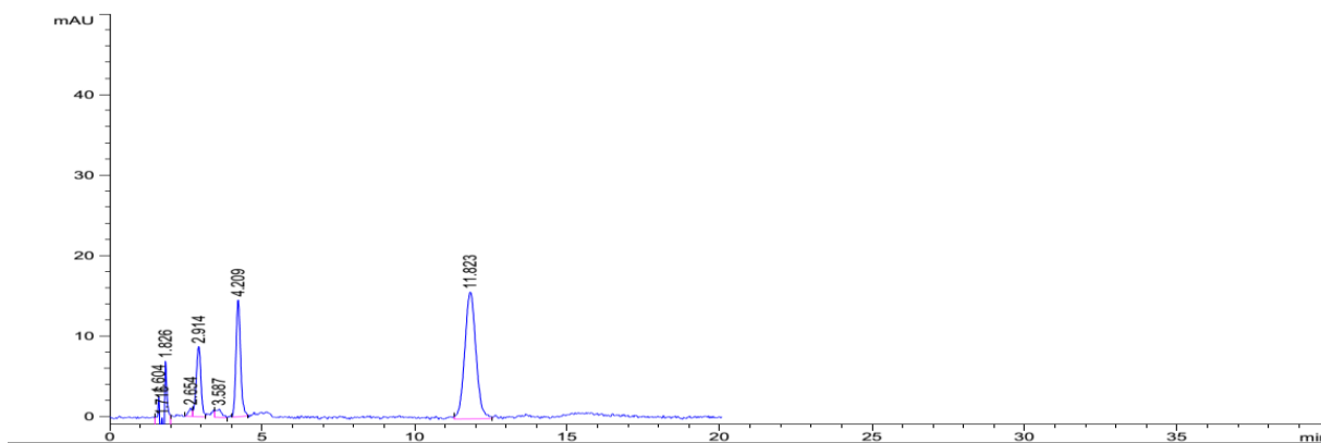
Fig. 3. HPLC chromatogram of lutein in leek.
