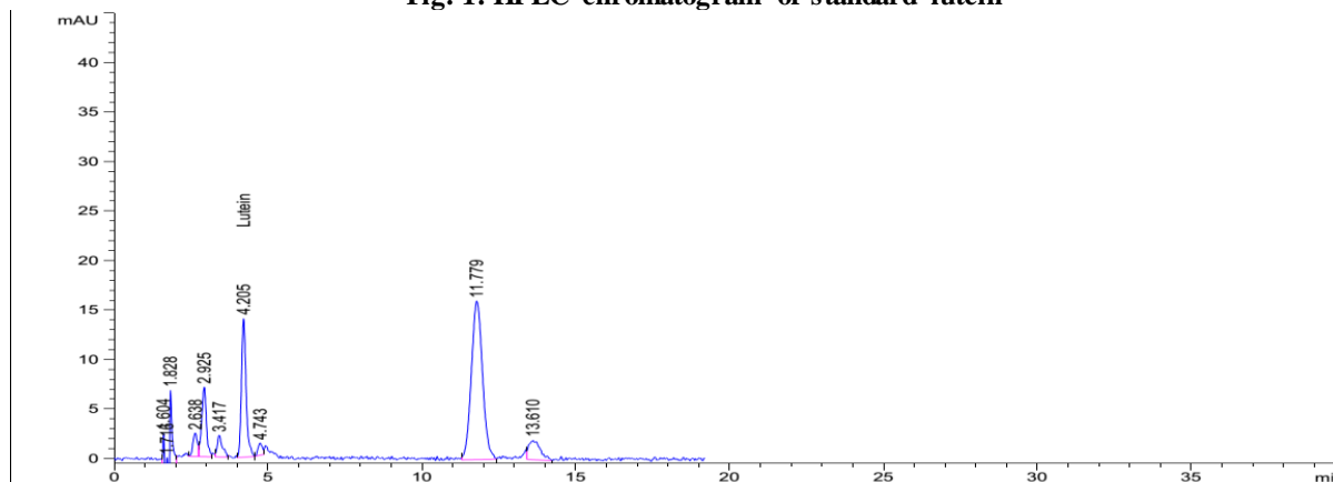
Fig. 2. HPLC chromatogram of lutein in spinach
