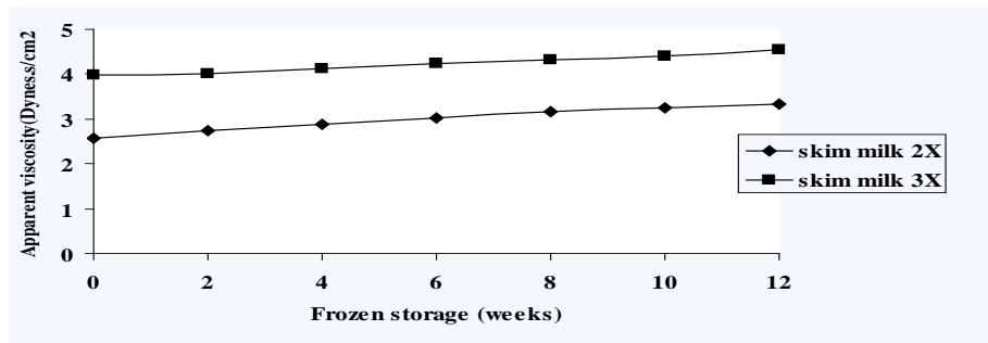
Fig. 4: Changes in apparent viscosity ( \eta_{app} ) value of frozen skim concentrated milk during storage at -22\text{ }^{\circ}\text{C} \pm 2 .
