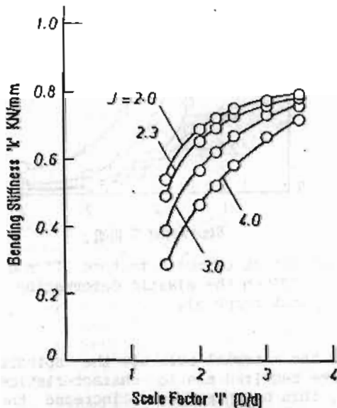
Fig.8 Effect of scale factors 'I' and 'J' on the bending stiffness.
