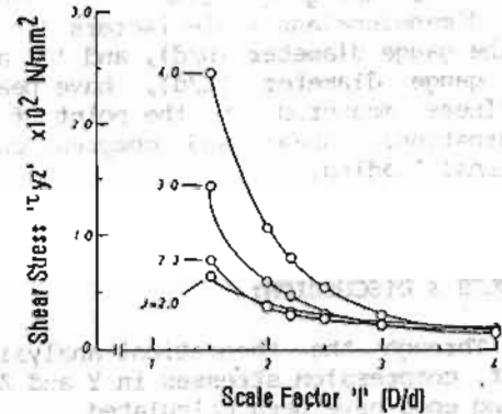
Fig.10 Effect of scale factors 'I' and 'J' on the shear stresses.
