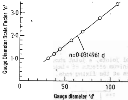
Fig.2 Relation between the scale factor 'n' and gauge diameters.
