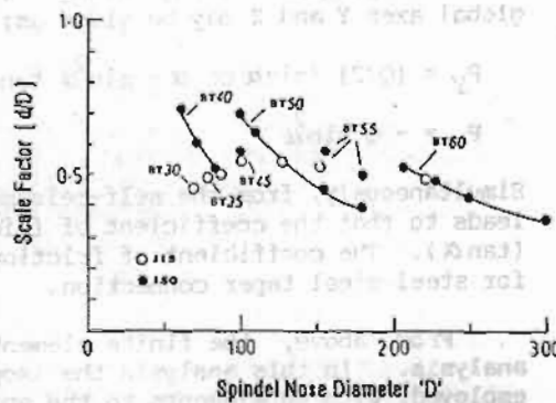
Fig.6 Relation between the scale factor 'd/D' and spindle nose diameters.
