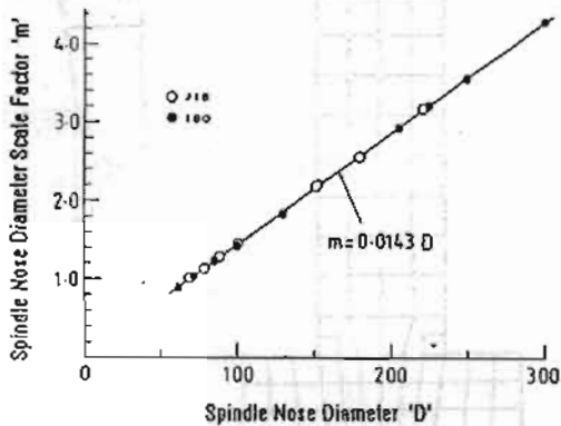
Fig.4 Relation between the scale factor 'm' and spindle nose diameters.
