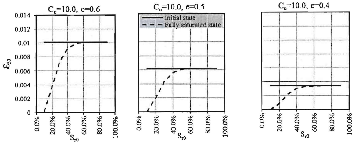
Fig. (13) Relation between ( \epsilon_{50} ), uniformity coefficient ( C_u=10 ), initial void ratio ( e ) and degree of saturation ( S_{10} )
