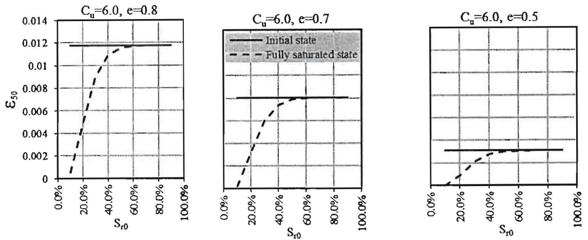
Fig. (12) Relation between ( \epsilon_{50} ), uniformity coefficient ( C_u=6.0 ), initial void ratio ( e ) and degree of saturation ( S_{10} )
