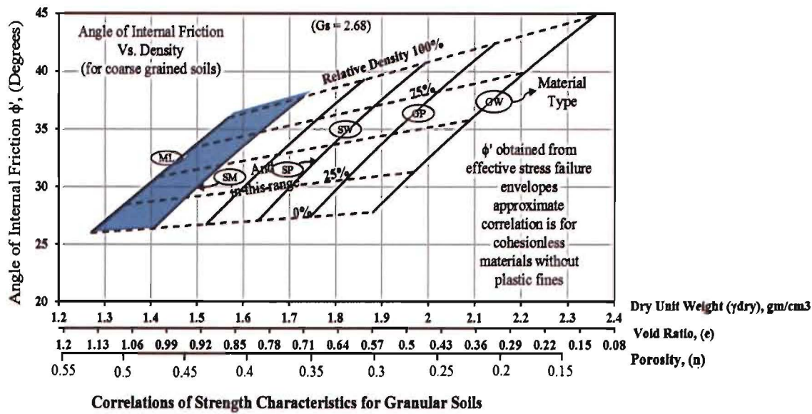
Fig. (6) Correlations of strength characteristics for granular soils (DM 7.01), 1986
