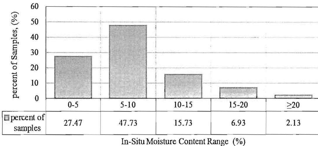
Fig. (3): Histogram of sampling in-situ water content
