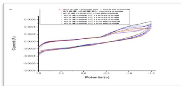
Fig (4). Cyclic voltammograms for interaction of 1mM of UO_2^{+2} in presence of 4-Flouro benzoic acid (FBA).
