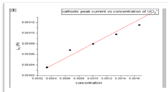
Fig. (2): Cathodic peak current against concentration of UO 2 2+ in 0.1 M HCl (0.1 M) at 291.95K
