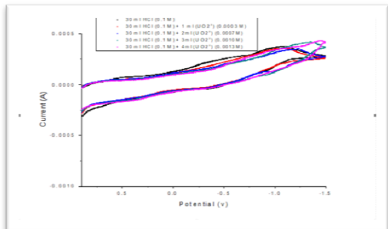
Fig.(1) Cyclic voltammogram of different concentrations of UO 2 2+ (0.0003, 0.0007, 0.001 and 0.0013) M at 291.95K.
