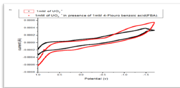
Fig (3). Cyclic voltammograms for interaction of 1mM of UO_2^{+2} in presence of 1mM (FBA).
