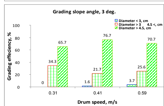
Fig. 7. Effect of drum speed on grading efficiency for Baladi eggplants variety eggplant
