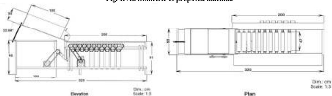
Fig. 2. Schematic diagram of the grading machine
