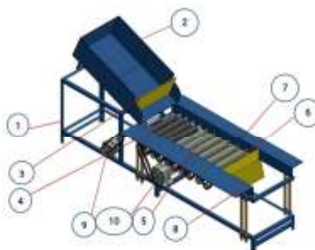
Fig. 1. An isometric of proposed machine
