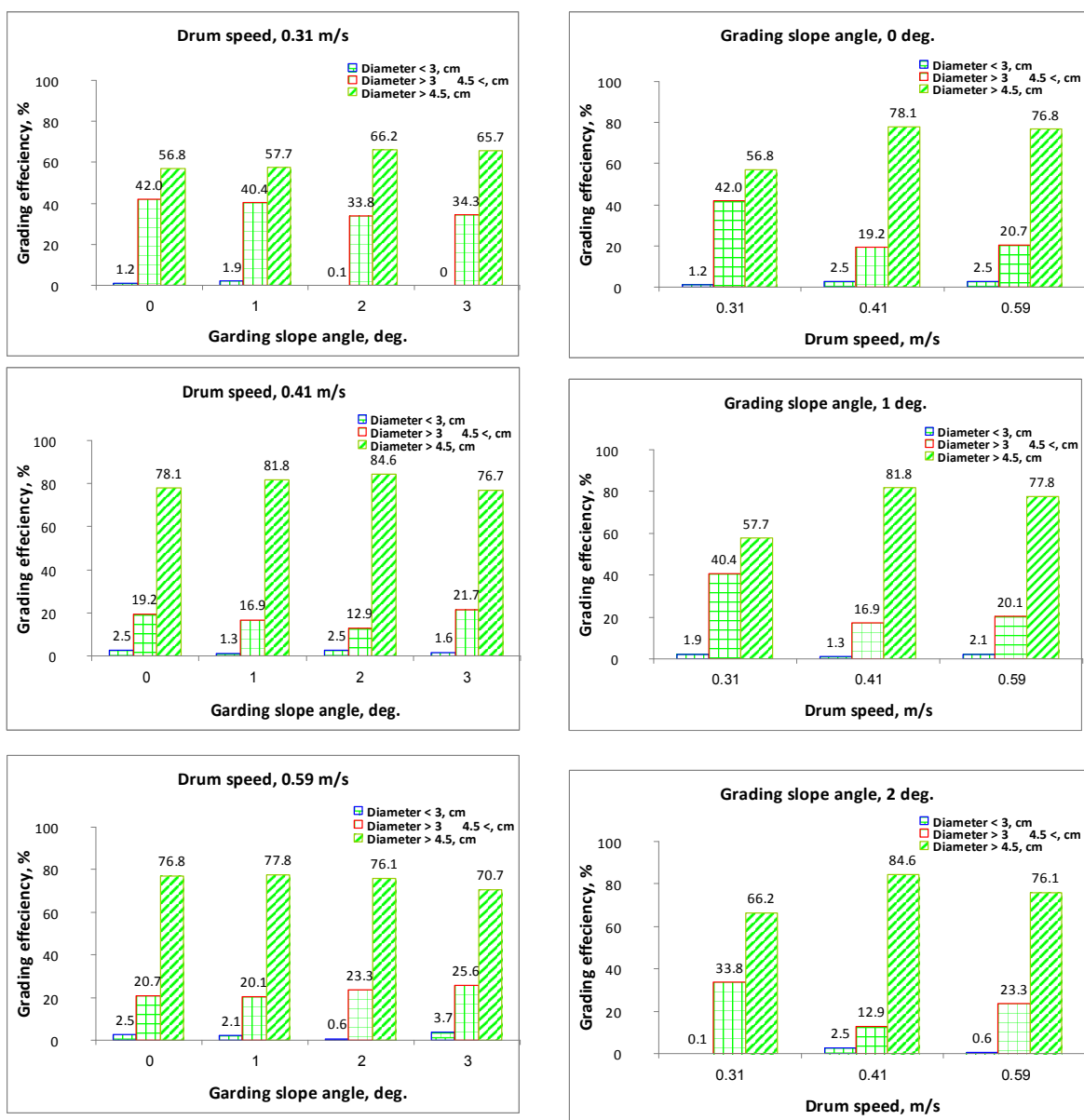
Fig. 6. Effect of grading slope angle on grading efficiency for Baladi eggplants variety eggplant
