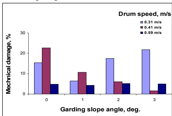
Fig. 8. Mechanical damage caused by the grading unit for Baladi eggplants variety eggplant
