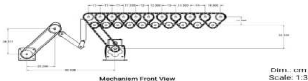
Fig. 3. The transmission system of the machine
