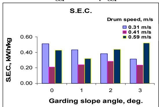
Fig. 9. Effect of drum speed and different slope angle deg. on the SEC for grading machine of Baladi eggplants variety eggplant
