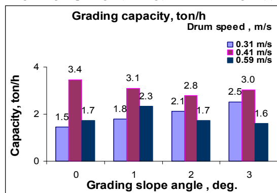
Fig. 5. Effect of drum speed and grading slope angle on grading capacity for Baladi eggplants variety eggplant
