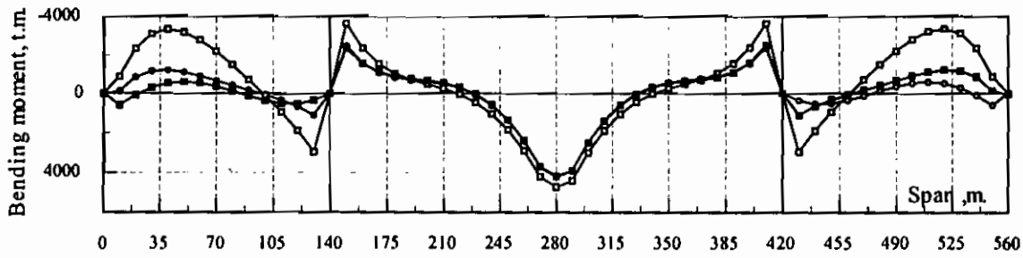
Fig(34): Bending moment in plane along floor beam(1) in three dimensional, case (B)
