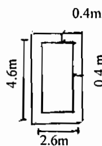
Fig. (1-d) : cross-section of pylons. A = 5.76 \text{ m}^2 , I_x = 17.88 \text{ m}^4 I_y = 7.5 \text{ m}^4 I_p = 0.4 \times 0.4 (2 \times 2.6 \times 2.6 \times 4.6 \times 4.6) / (2.6 \times 0.4 + 4.6 \times 0.4) = 15.9 \text{ m}^4
