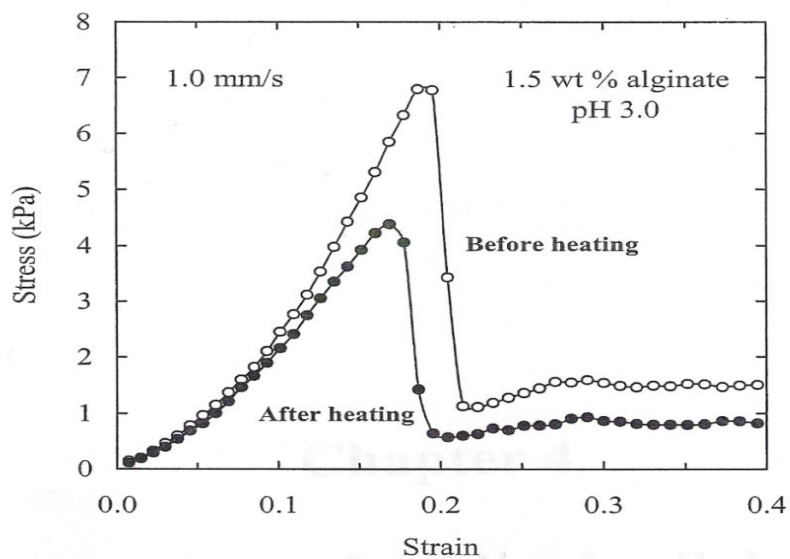
Fig. 11. Compression curves (1.0 mm/s) for 1.5 wt % alginate acidified with GDL to a final pH of 3.0, recorded at 25°C before (O) and after (●) heating to 85°C.
