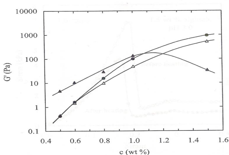
Fig.10. Variation of G' ( 1 \text{ rad s}^{-1} ; 0.5 % strain) with alginate concentration ( c ) for samples acidified with GDL to a final pH of 3.0, after reaching constant moduli at 25°C (●), on reaching 85°C after heating at 1°C/min ( \Delta ), and after cooling back to 25°C at 1°C/min ( \blacktriangle ).
