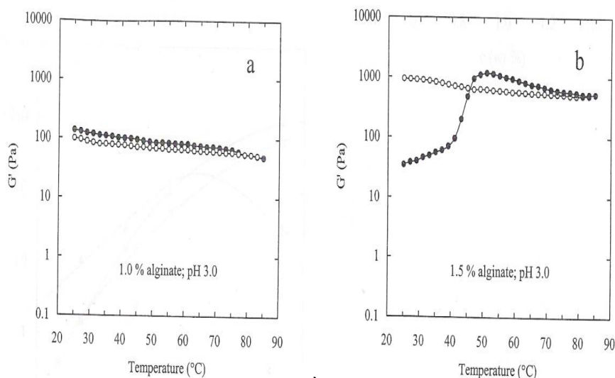
Fig. 9. Values of G' ( 1 \text{ rad s}^{-1} ; 0.5 % strain) recorded during heating (O) and cooling (●) at 1^{\circ}\text{C}/\text{min} for samples acidified with GDL to a final pH of 3.0 at alginate concentrations of (a) 1.0 wt % and (b) 1.5 wt %.
