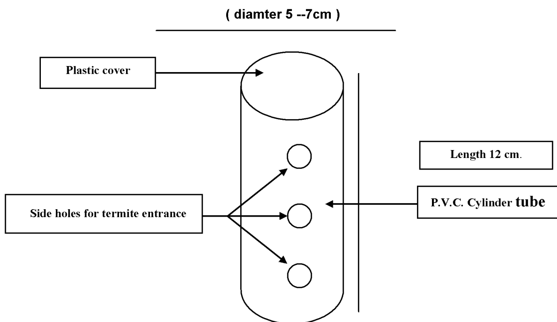
Fig. (1): Description of the developed subterranean termites trap.
