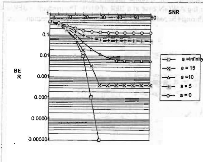
Figure 11. Performance of OFDM/DE 16 star QAM, single source per channel multiplexing in AWGN with first fading channel (Rician fading).
